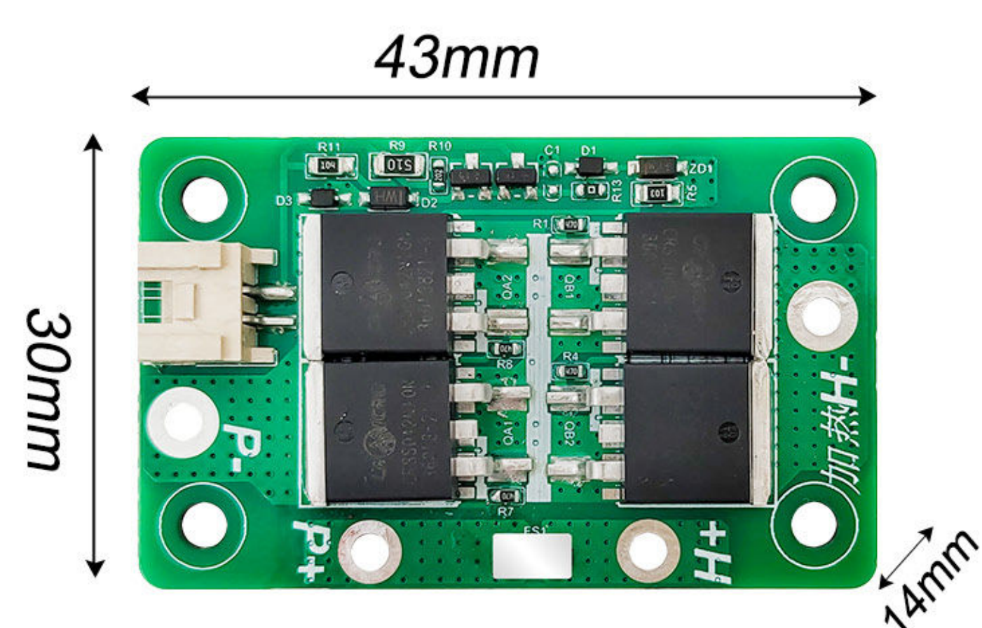
Heating module
