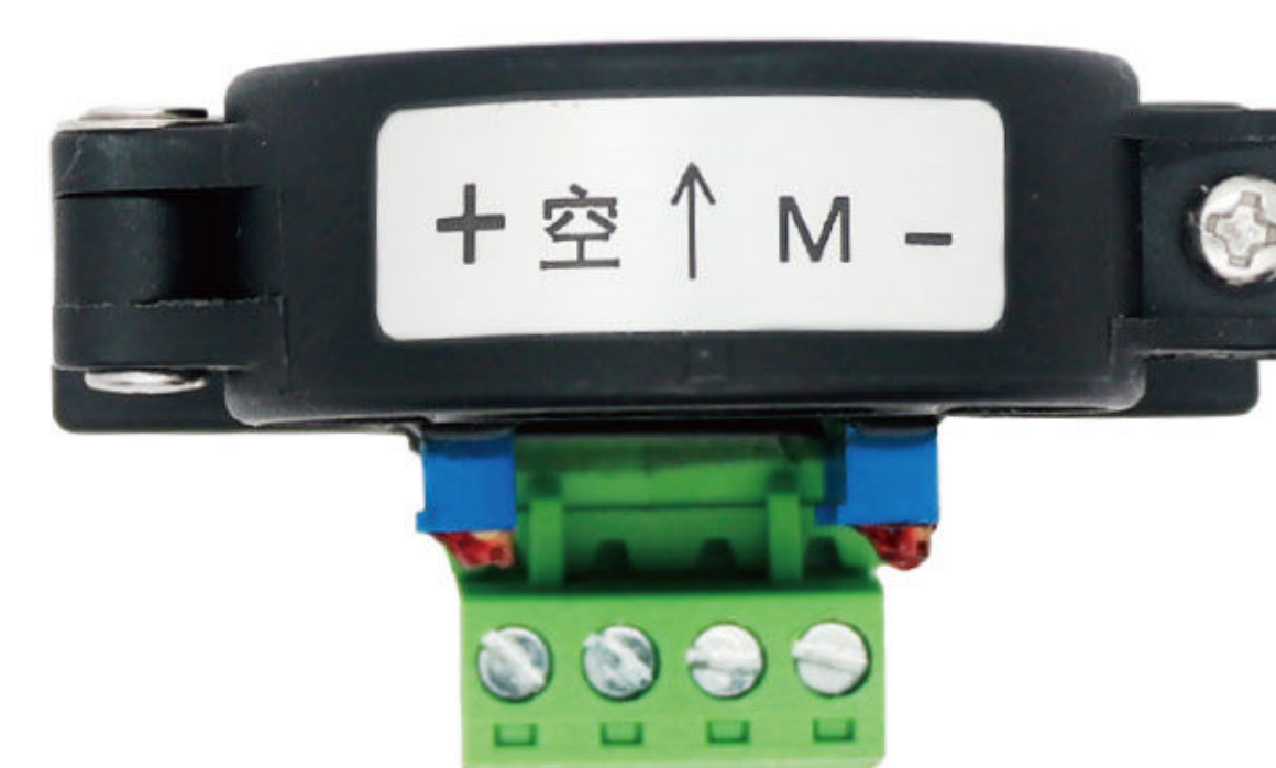
Hall sensor
